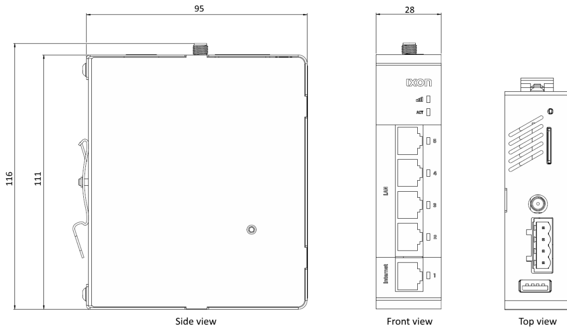
Figure 3: IXrouter3 dimensions
