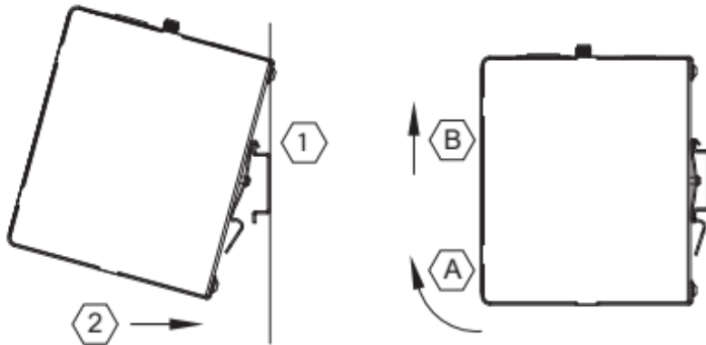
Figure 4: DIN-rail installation
